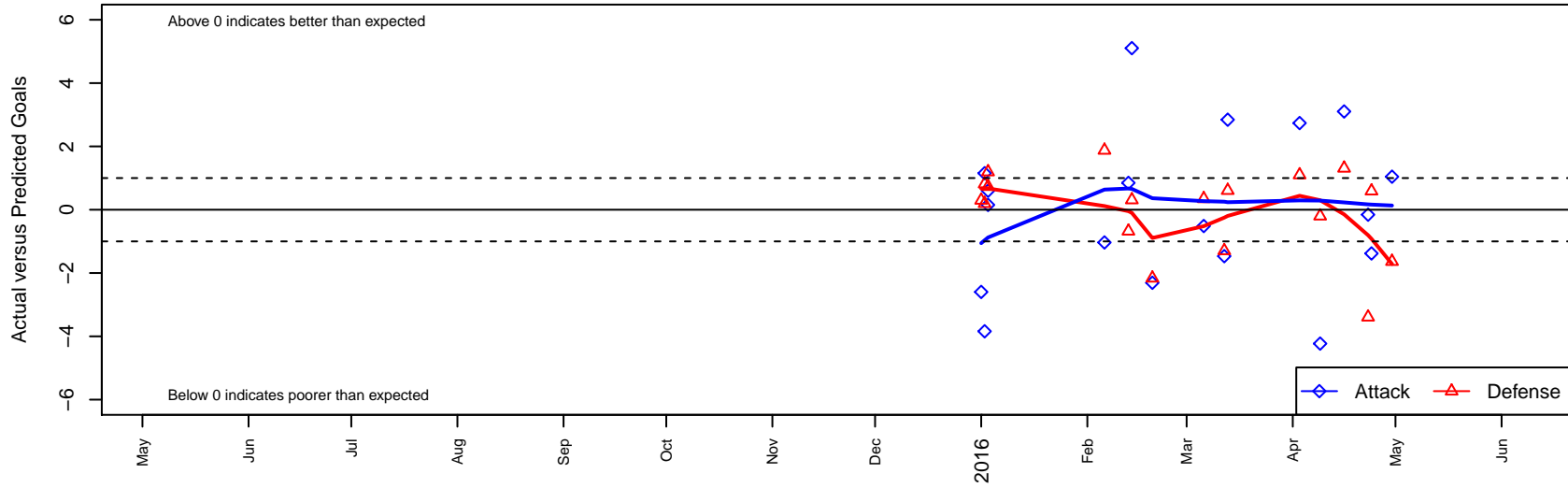
LASC Eagles B04 Dots are actual minus expected GF (blue circles) and GA (red triangles). Blue line is smoothed change in attack strength. Red is smoothed change in defense strength.
